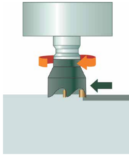
Material : Steel FACE MILLING
